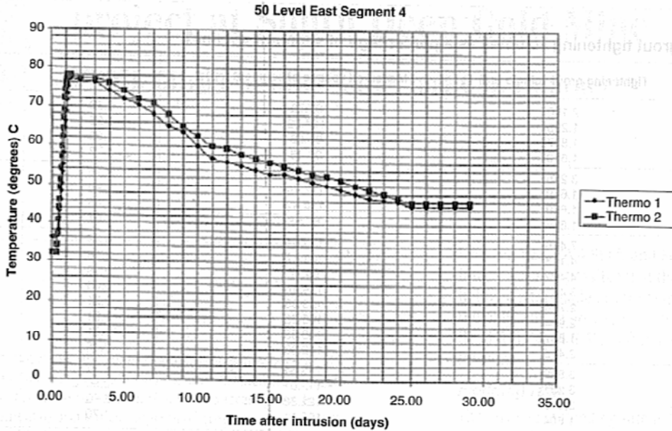
Figure 3—Temperature after Intrusion
